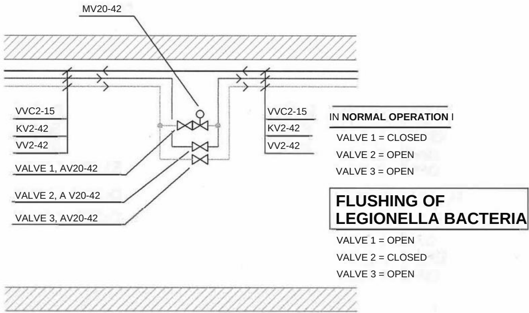
PRINCIPLE SECTION a - a OWN SCALE
