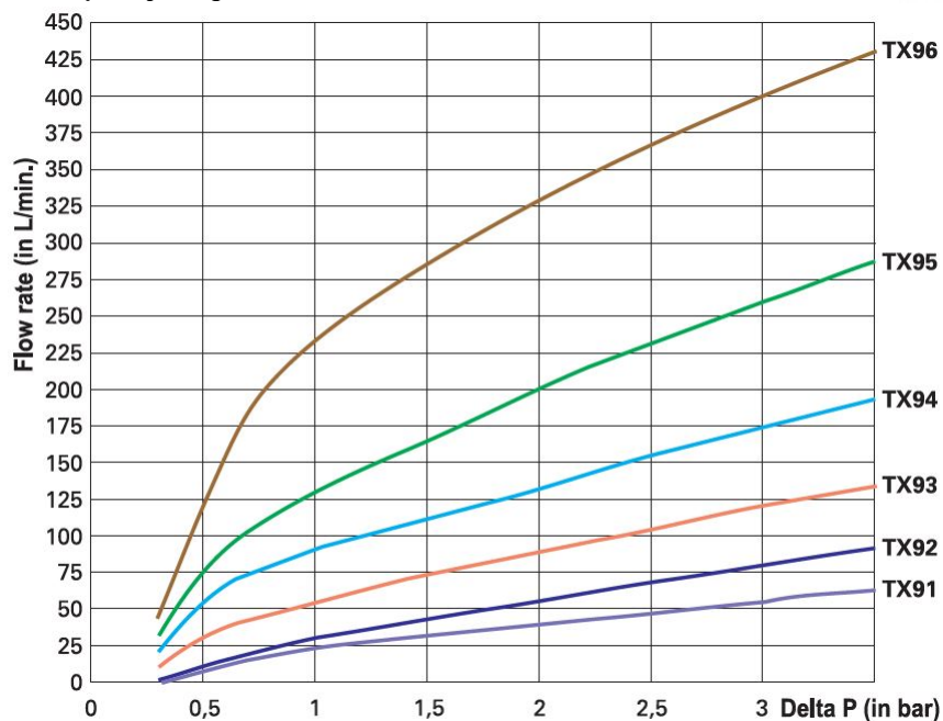
Capacity diagram Ultramix FNC
